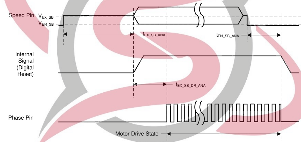
Figure 3. DRV10983SQ Analog Mode Timing
