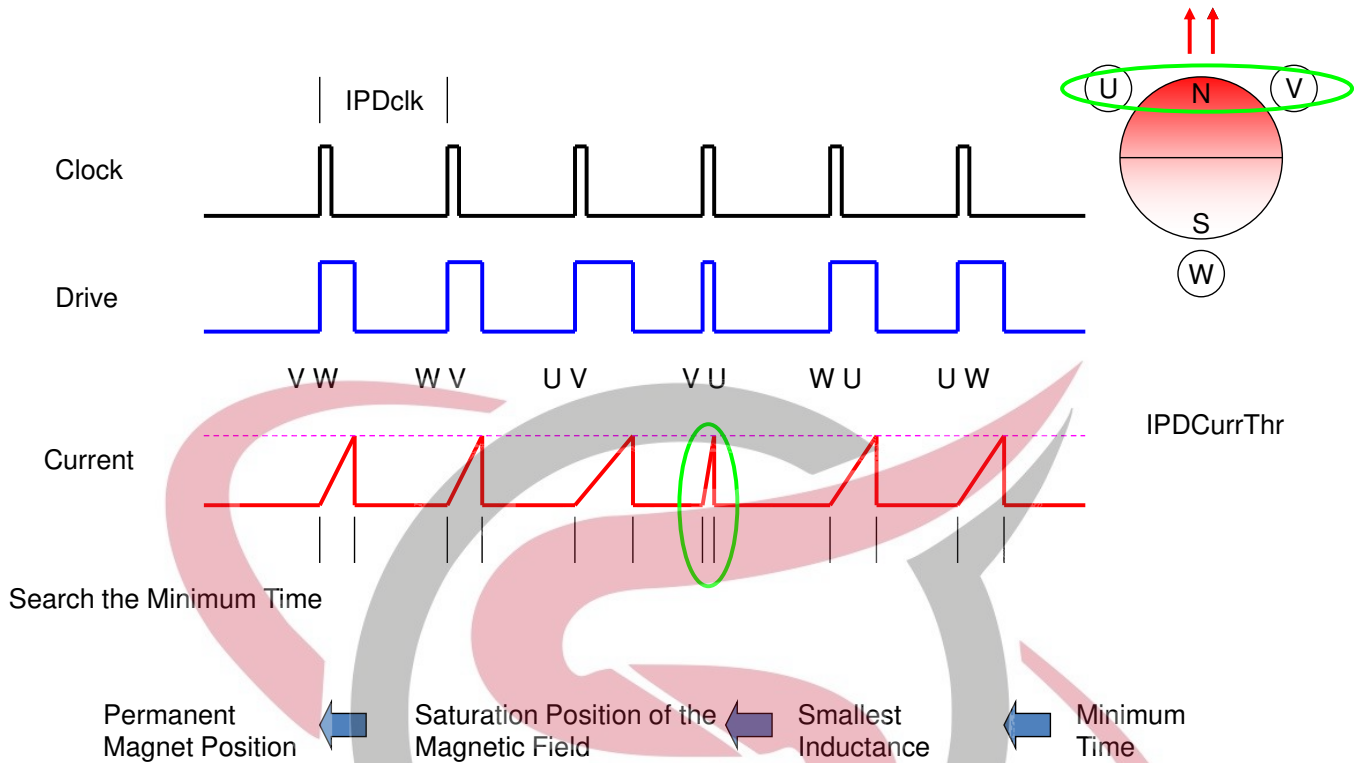
Figure 20. IPD Function
