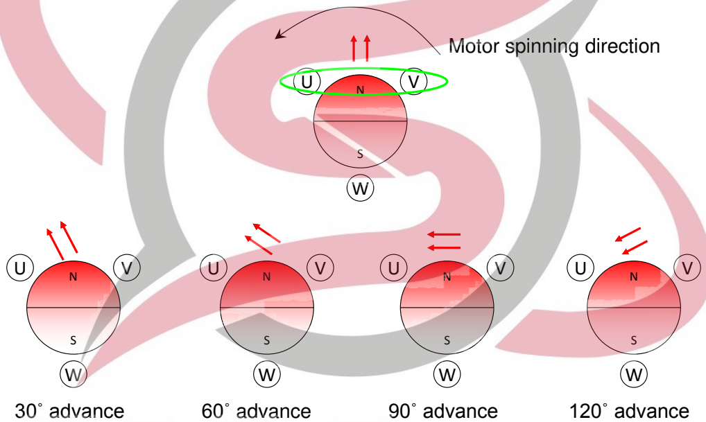
Figure 23. IPD Advance Angle
