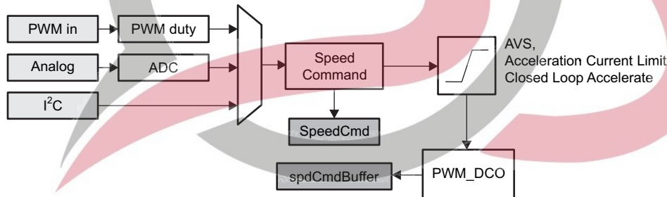
Figure 44. SpeedCmd and spdCmdBuffer Registers
