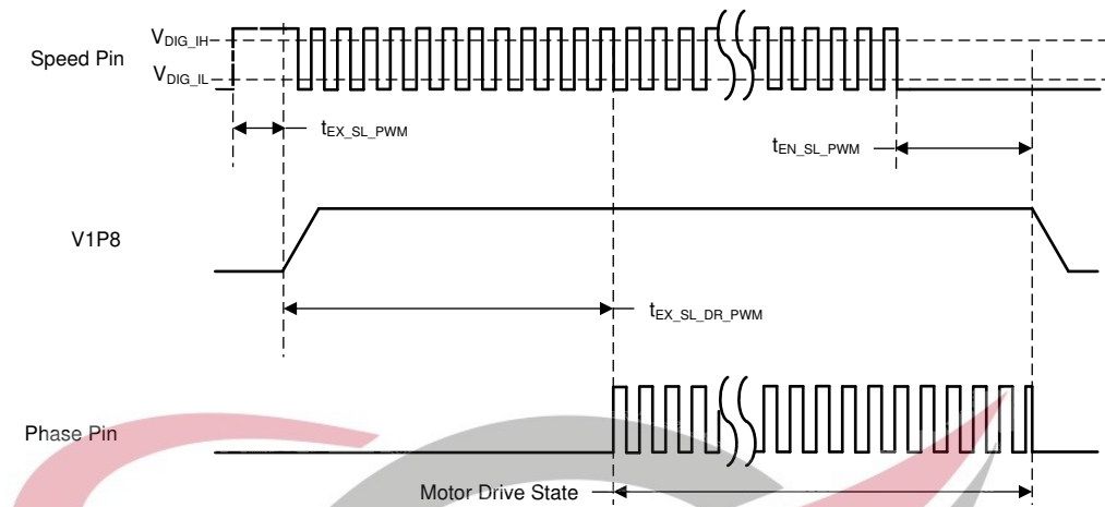
Figure 2. DRV10983Q PWM Mode Timing
