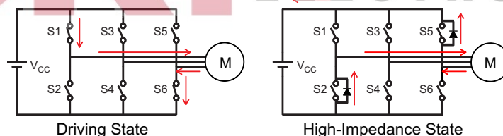
Figure 40. Inductive-Mode Voltage Surge
