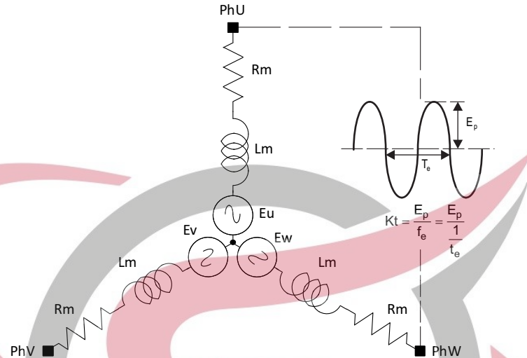
Figure 15. K_{tPH} Definition
